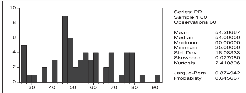
Figure (4) The Signing Graph of the Time Series of the Payout Ratio (PR)
