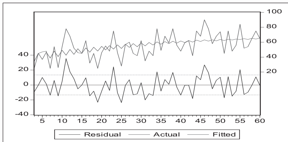
Figure (5) Signing Graph of Residual, Actual and Fitted Values of the Payout Ratio (PR) Time Series
